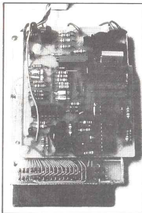
Decoder board (above). There's not much to it. This unit interfaces the project to the VZ200 and contains software in EPROM. Modem board (left). The receiver demodulator and transmitter modulator are contained on this board, mounted on the rear of the decoder board. Note the indicator LED.
